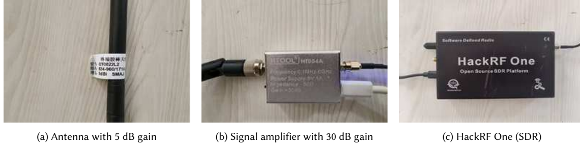
Fig. 4. Hardware components of the EMGesture prototype.
