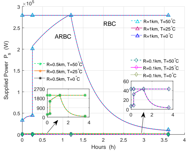
Fig. 15: Supplied Power with Different Radius and Temperature for 810 nm (Fog)
