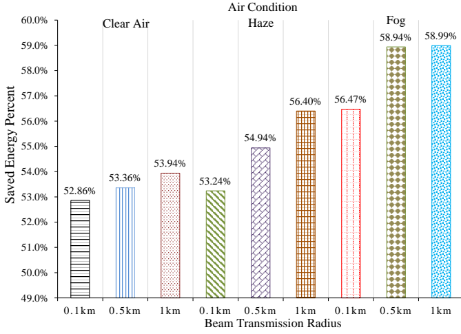
Fig. 22: The Percent of Saved Supplied Energy under 0°C ( \lambda=1550 nm)
