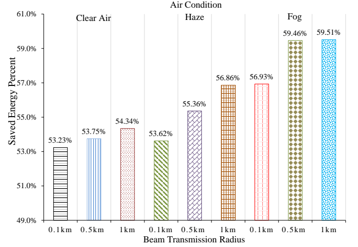
Fig. 20: The Percent of Saved Supplied Energy under 25°C ( \lambda=810 nm)
