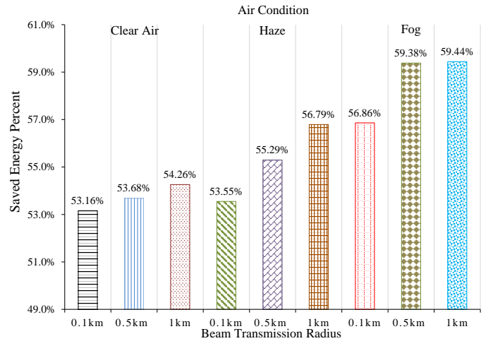
Fig. 21: The Percent of Saved Supplied Energy under 50°C ( \lambda=810 nm)
