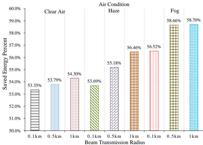
Fig. 24: The Percent of Saved Supplied Energy under 50°C ( \lambda=1550 nm)
