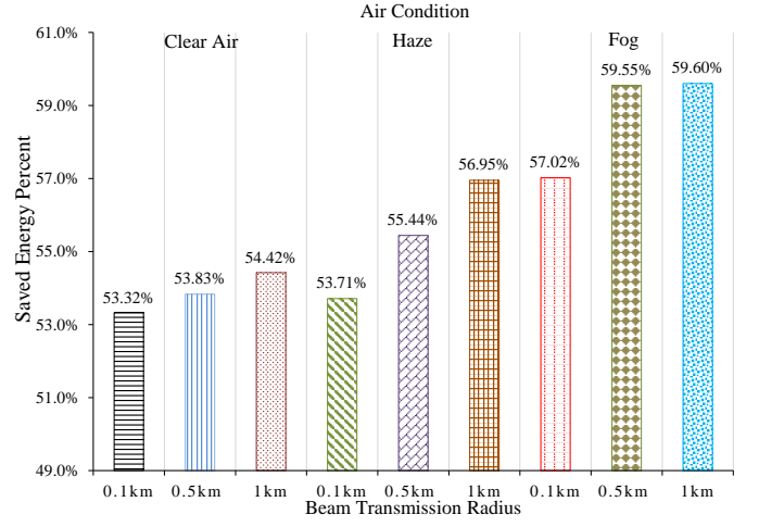
Fig. 19: The Percent of Saved Supplied Energy under 0°C ( \lambda=810 nm)
