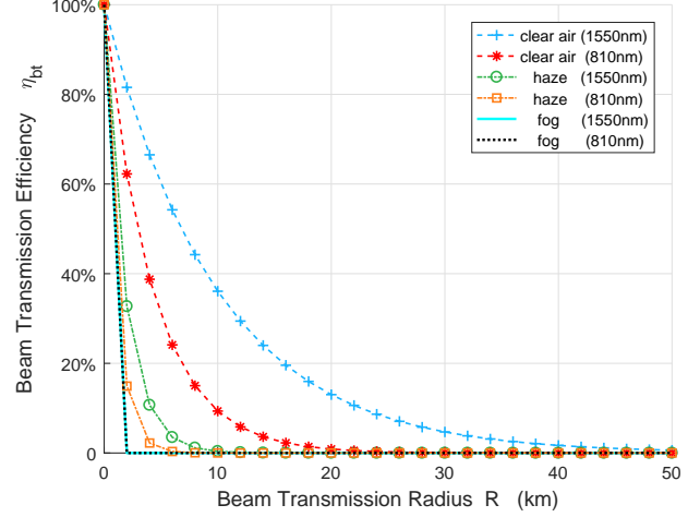
Fig. 7: Beam Transmission Efficiency vs. Radius
