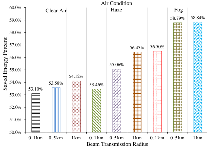
Fig. 23: The Percent of Saved Supplied Energy under 25°C ( \lambda=1550 nm)
