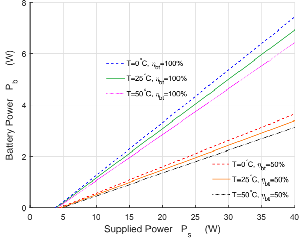
Fig. 11: Battery Power vs. Supplied Power (1550 nm)
