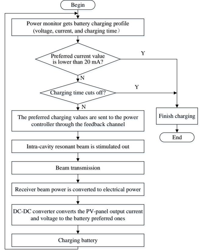
Fig. 3: ARBC Flow Chart
